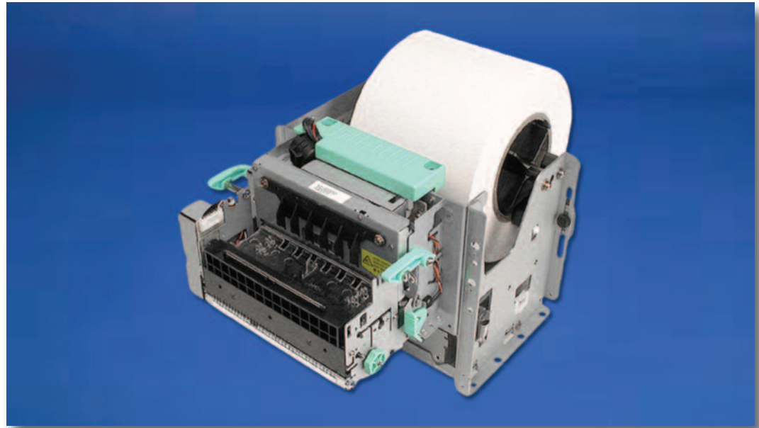
Optional 10" Diameter Paper Roll holder
